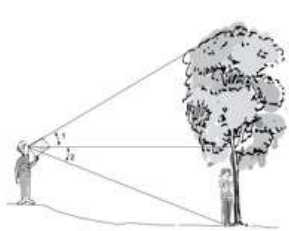
III. Two Triangles with Eyes Higher Than Tree Base
