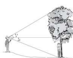
III. Two Triangles with Eyes Higher Than Tree Base
