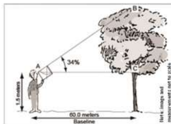
I. Standard Clinometer Technique
