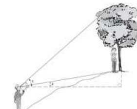
IV. Two Triangles with Eyes Lower Than Tree Base
