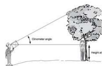
V. Stand by Tree Technique
