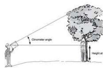
V. Stand by Tree Technique
